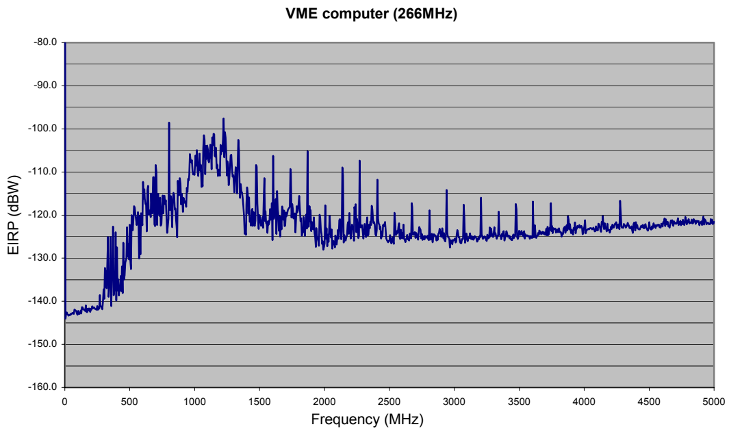
A computer with a VME bus structure and a 266MHz processor.
